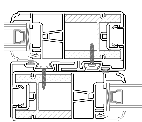
6 Meeting Rail Detail
